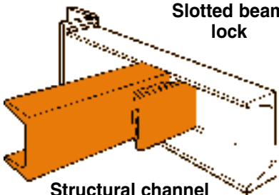
Structural channel pallet support
